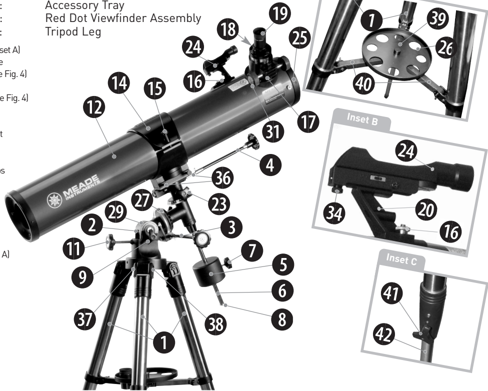
Figure 1: Meade 114EQ-AR Equatorial Reflecting Telescope
