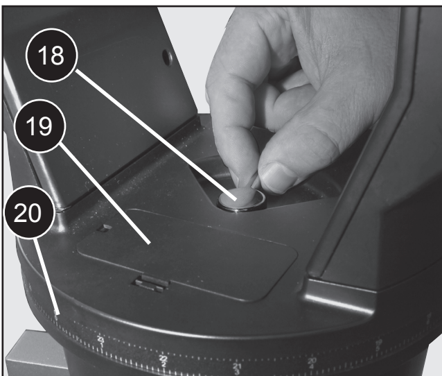
Figure 15: ETX 90 Top of Base
