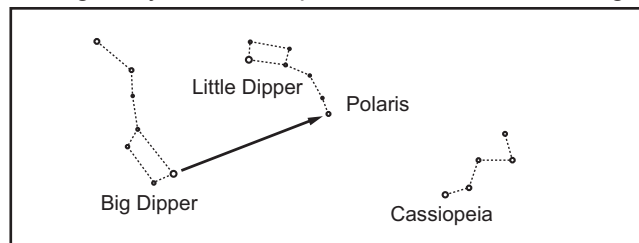
Figure 30: Locating Polaris
