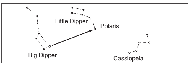
Figure 2: Locating Polaris
